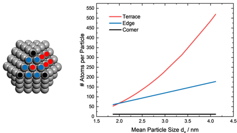
Fig. 2 Number of variously coordinated surface atoms, C_5 (corners), C_7 (edges), C_8 + C_9 (terraces), in an ideal cuboctahedral platinum particle. Calculated from Kaatz et al. 21
